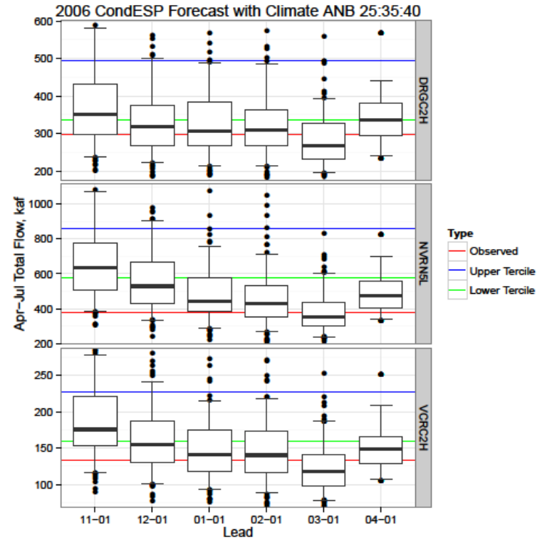
Figure B.4 Boxplots of Seasonal Volume Totals for the CondESP streamflow forecasts for 2005 and 2006. The observed value for each year is the red line, while the climatological upper and lower terciles are shown in blue and green, respectively.
