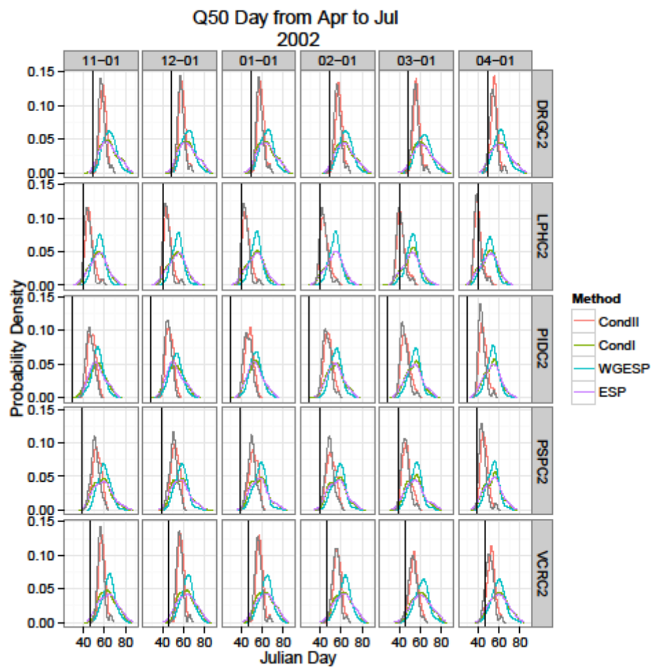
Figure 1.21 Q50 Julian Day between April and May for 2002 simulated using the synthetic climate forecasts.
