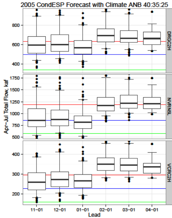
Figure B.4 Boxplots of Seasonal Volume Totals for the CondESP streamflow forecasts for 2005 and 2006. The observed value for each year is the red line, while the climatological upper and lower terciles are shown in blue and green, respectively.
