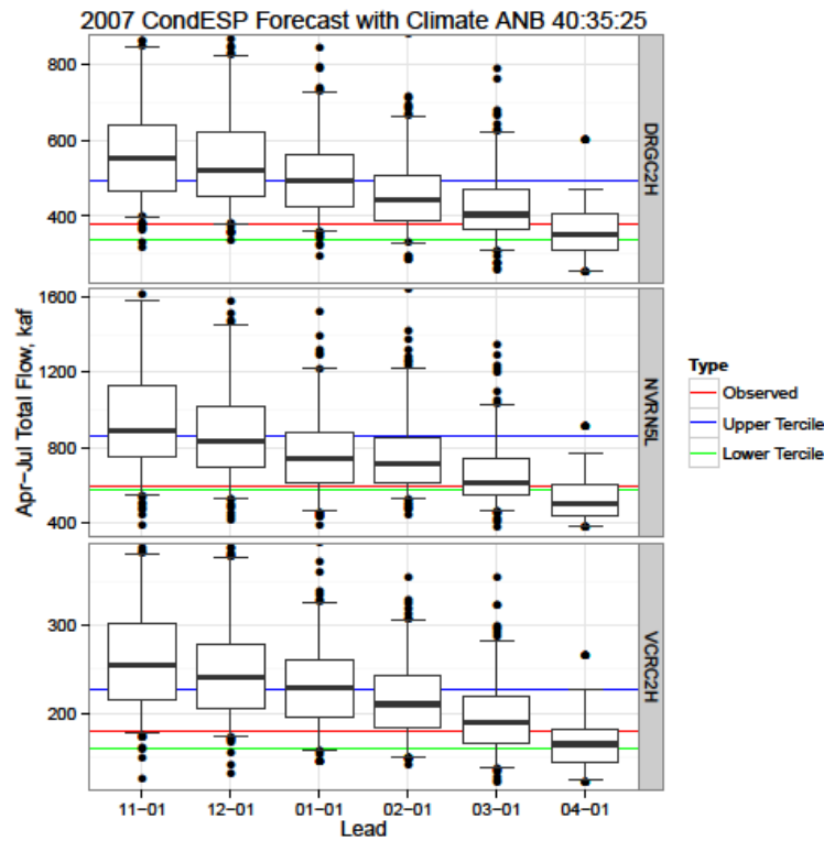
Figure B.5 Boxplots of Seasonal Volume Totals for the CondESP streamflow forecasts for 2007 and 2008. The observed value for each year is the red line, while the climatological upper and lower terciles are shown in blue and green, respectively.
