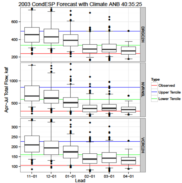
Figure B.3 Boxplots of Seasonal Volume Totals for the CondESP streamflow forecasts for 2002 and 2003. The observed value for each year is the red line, while the climatological upper and lower terciles are shown in blue and green, respectively.
