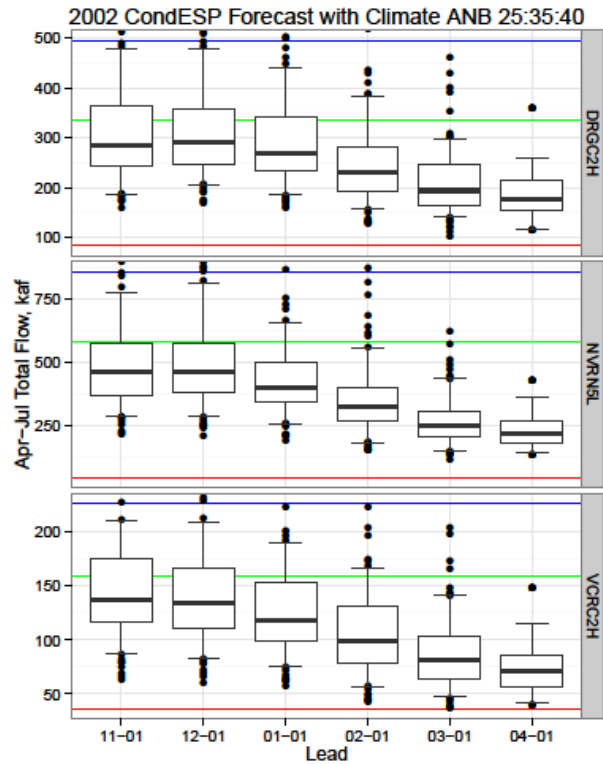
Figure B.3 Boxplots of Seasonal Volume Totals for the CondESP streamflow forecasts for 2002 and 2003. The observed value for each year is the red line, while the climatological upper and lower terciles are shown in blue and green, respectively.
